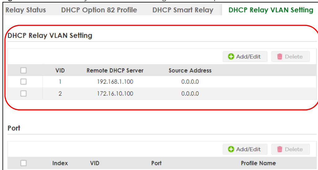
Figure 247 DHCP Relay for Two VLANs Configuration Example
