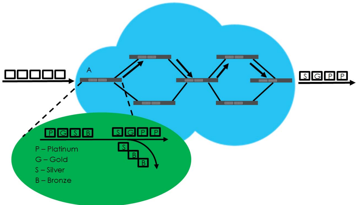
Figure 184 DiffServ Network
